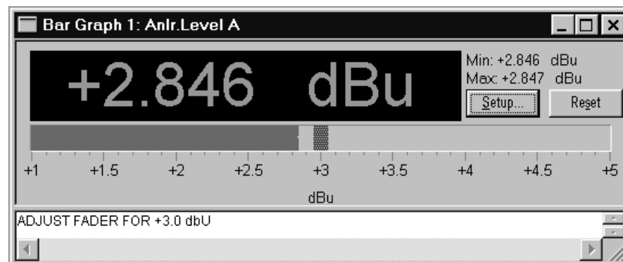
Figure 21-11 Readings Bargraph, Showing Max-min Bar, Target Area, and Prompting Message (Comment) to Operator
