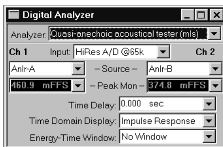
Figure 17-2 MLS Panel, small form
