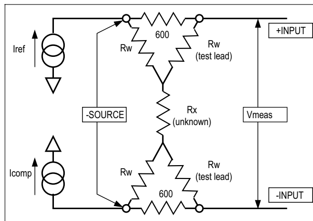
Figure 26-6 Simplified diagram of 4-wire ohmmeter operation
