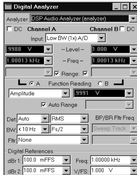
Figure 11-2 DSP Audio Analyzer Panel, Large Form
