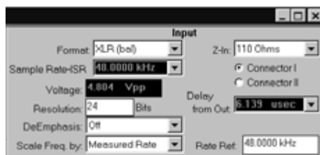
Figure 7-1 Input Controls on Large Version of Digital Input-Output Panel
