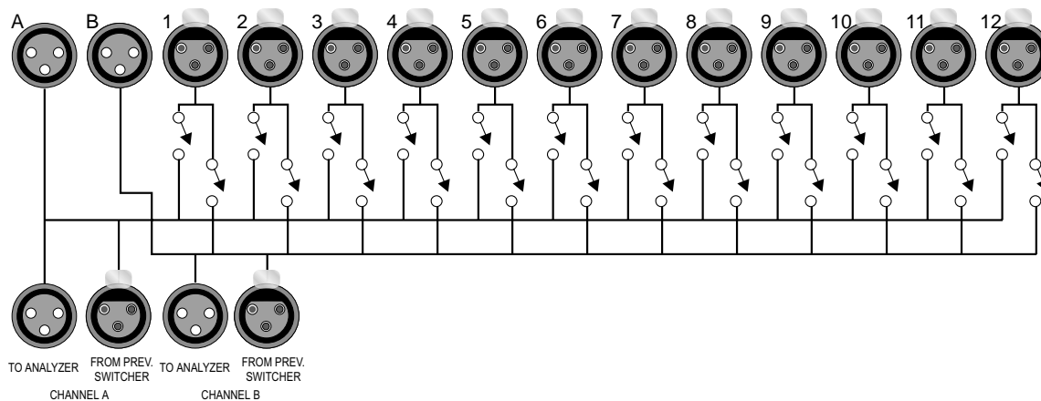
Figure 25-5 Input Switcher simplified schematic
