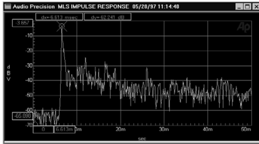
Figure 17-3 Loudspeaker Impulse Response, Showing 6.6 Millisecond Delay to Impulse Peak. This Waveform Furnished as C:\APWIN\S1\PROCEDURE\DEMO\THREWAY.AAM
