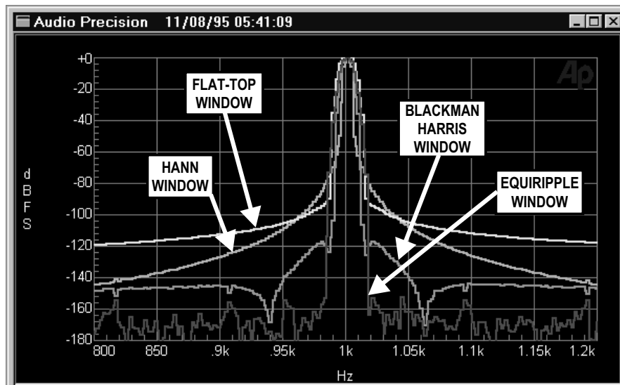
Figure 15-3 Available Window Functions, FFT
