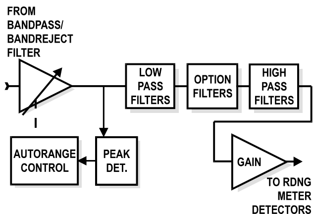
Figure 5-22 System Two Analog Analyzer, Simplified Block Diagram of Fixed Filter
