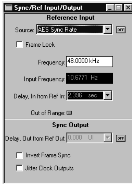
Figure 18-1 Sync-Ref Panel
