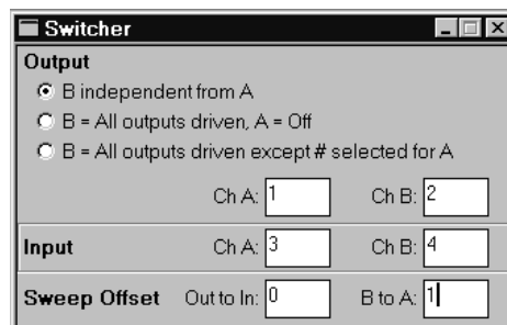
Figure 25-1 Switcher Panel
