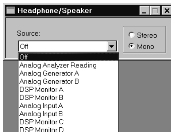
Figure 3-3 Headphone/Speaker Panel
