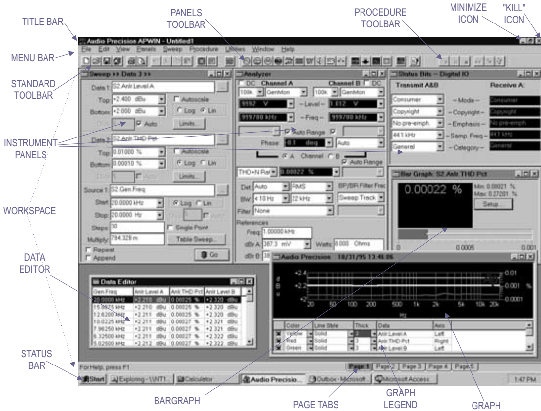
Figure 2-1 APWIN Screen
