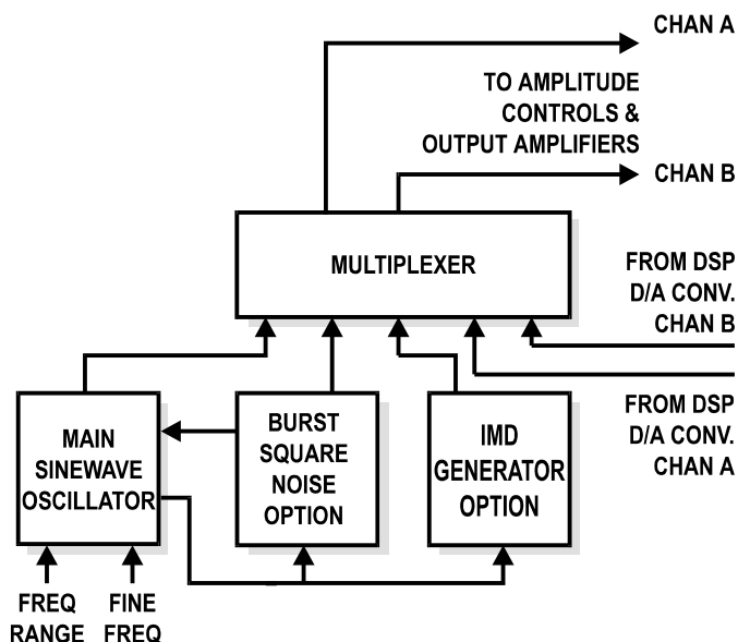
Figure 4-15 Oscillator Section, System Two Analog Generator
