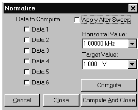
Figure 23-2 Compute Normalize Dialog
