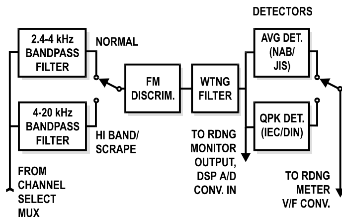
Figure 5-8 Wow and Flutter Analyzer Option, Simplified Diagram
