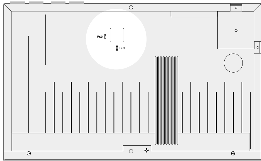
Figure 25-16 P62 and P63 Jumper Locations Inside SWR-2122 Switchers
