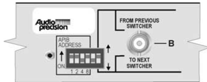
Figure 25-19 Unbalanced switcher address/mode switch
