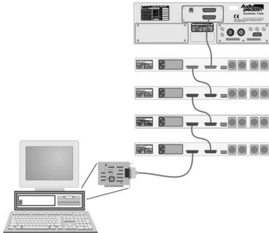
Figure 25-15 APIB connections block diagram (typical)
