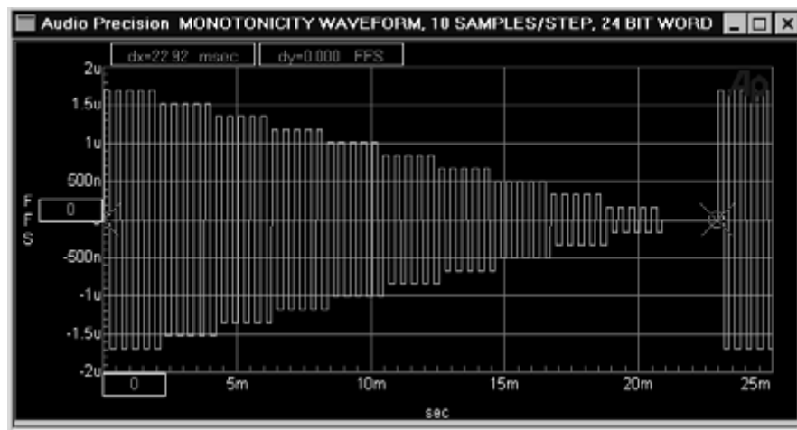
Figure 10-6 Monotonicity Waveform with 24-Bit Word Width, 10 Samples/Step, 48 kHz Sample Rate
