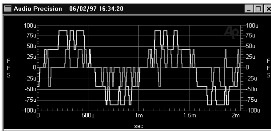
Figure 15-9 -85 dBFS and -100 dBFS 16-bit sine wave signals, normal dither, no averaging.
