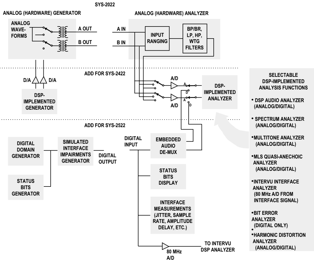
Figure 1-1 Conceptual Block Diagram, System Two
