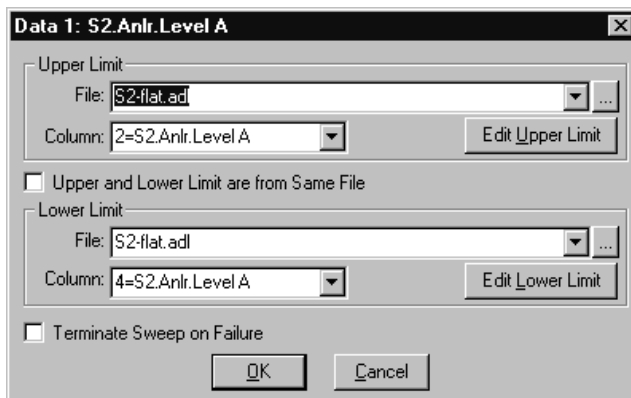
Figure 22-5 Limits Dialog, Obtained via Limits Button for each Data Parameter. Note Edit Upper Limit and Edit Lower Limit Buttons to Display Attached File Editor
