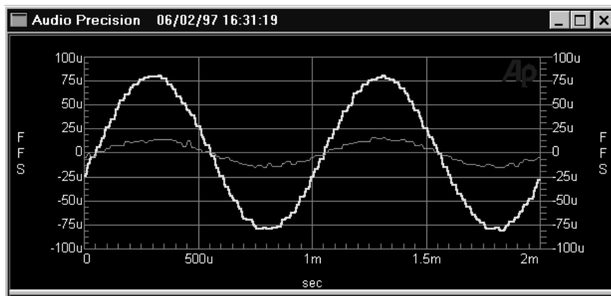
Figure 15-10 -85 dBFS and -100 dBFS 16-bit sinewave signals, normal dither, 256x synchronous averaging, DGen triggering
