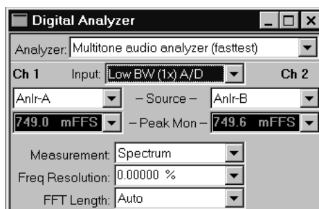
Figure 16-2 Multitone Audio Analyzer (FASTTEST), small version
