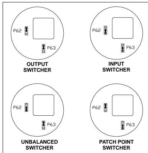
Figure 25-17 P62 and P63 Jumper Placement for Output, Input, Patch Point, and Unbalanced Switchers
