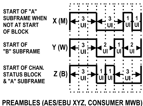
Figure 8-4 Preambles
