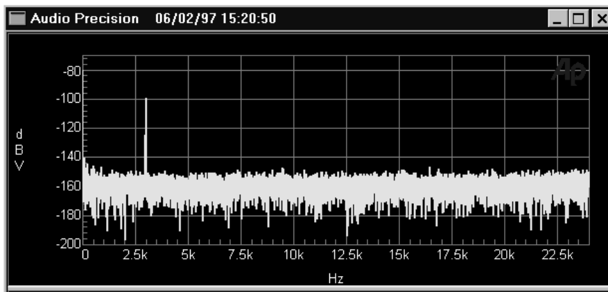
Figure 15-6 Low Level Signal, No Averaging
