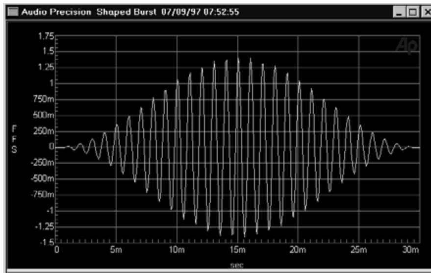
Figure 10-4 Shaped Burst of 1 kHz Frequency, 30 Cycles Duration
