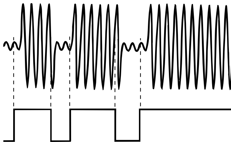
Figure 4-7 Burst Gated Mode, Definitions
