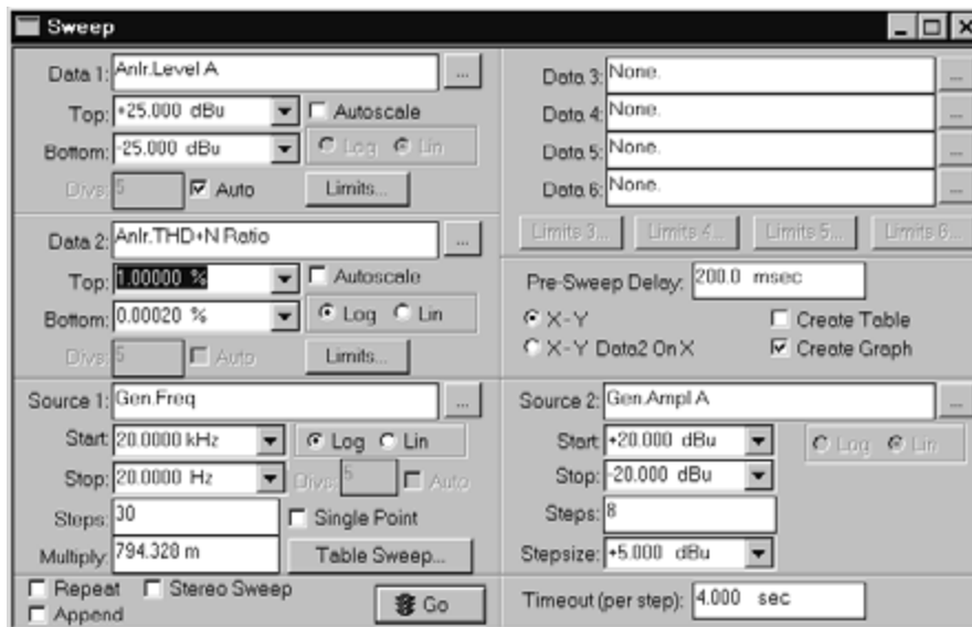
Figure 20-2 Sweep Panel, Large Version
