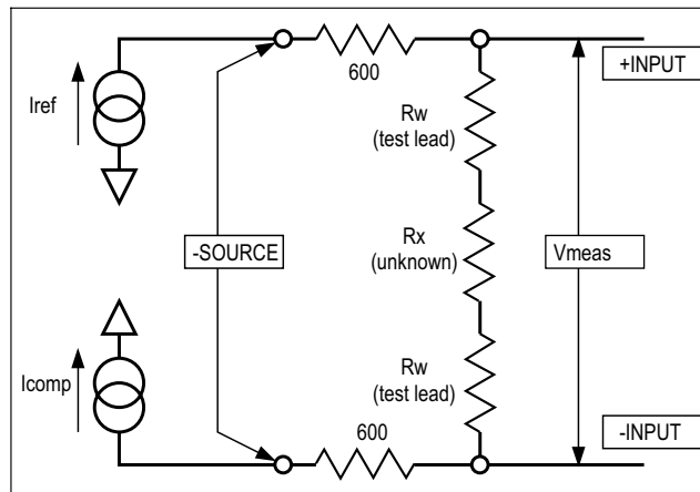
Figure 26-5 Simplified diagram of 2-wire ohmmeter operation
