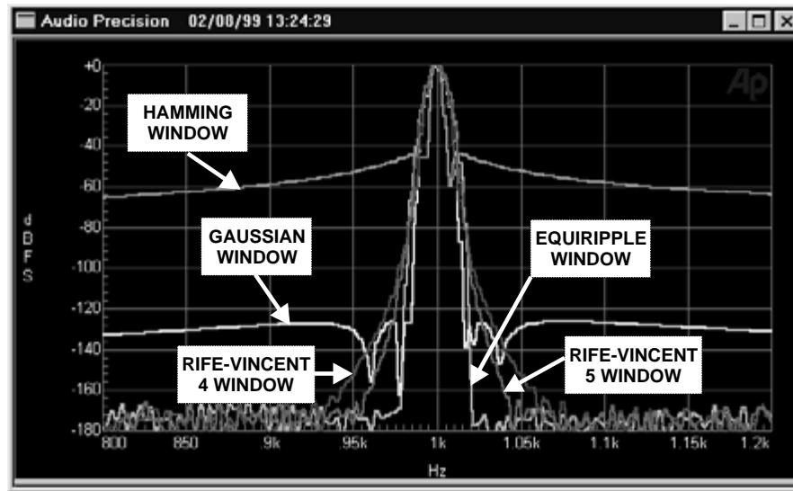
Figure 15-4 Additional Window Functions Available with System Two Cascade, FFT; Equiripple Shown in Both Figures for Comparison
