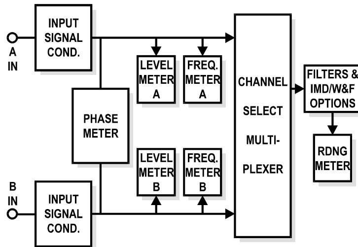
Figure 5-17 System Two Analog Analyzer, Simplified Block Diagram
