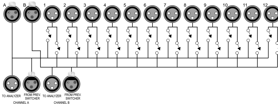
Figure 25-8 Output Switcher simplified schematic
