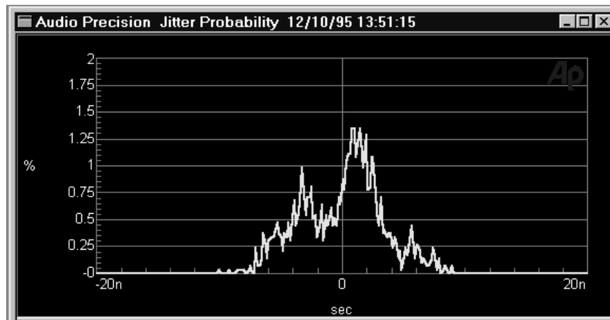
Figure 8-16 Jitter Probability
