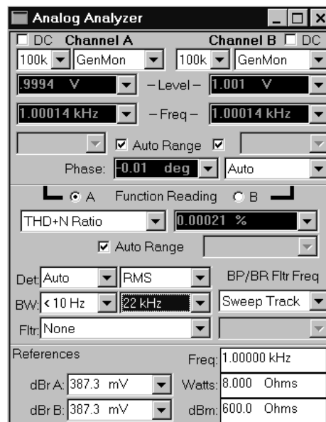
Figure 5-2 System Two Analog Analyzer Panel, Large Version
