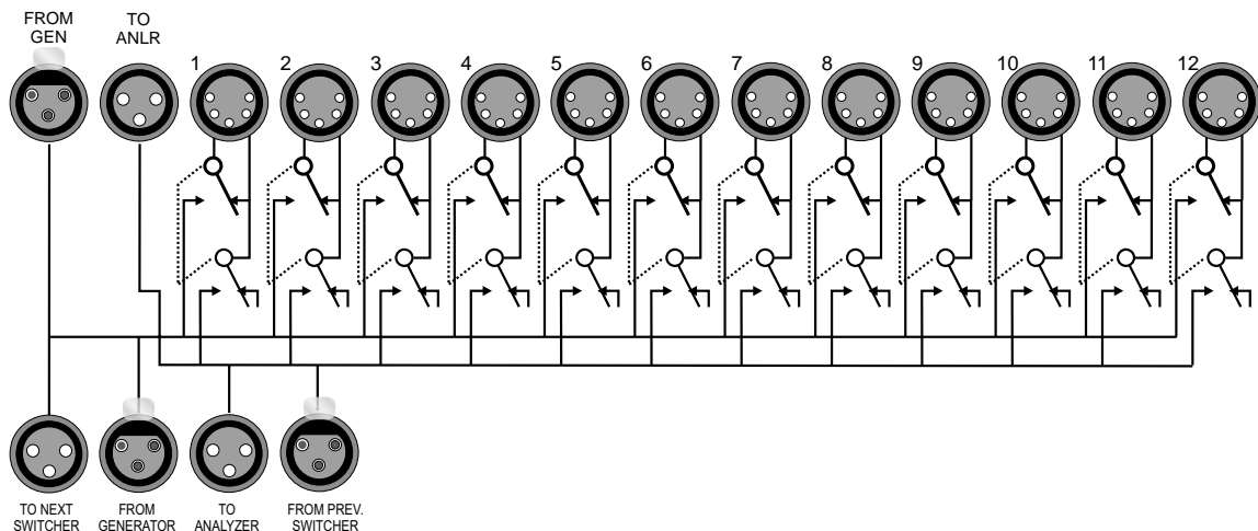
Figure 25-14 SWR-2122P Patch-Point Switcher simplified schematic
