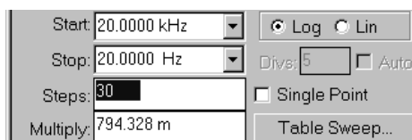
Figure 20-5 Log Sweep; Resolution Value is Constant “Multiply” Value
