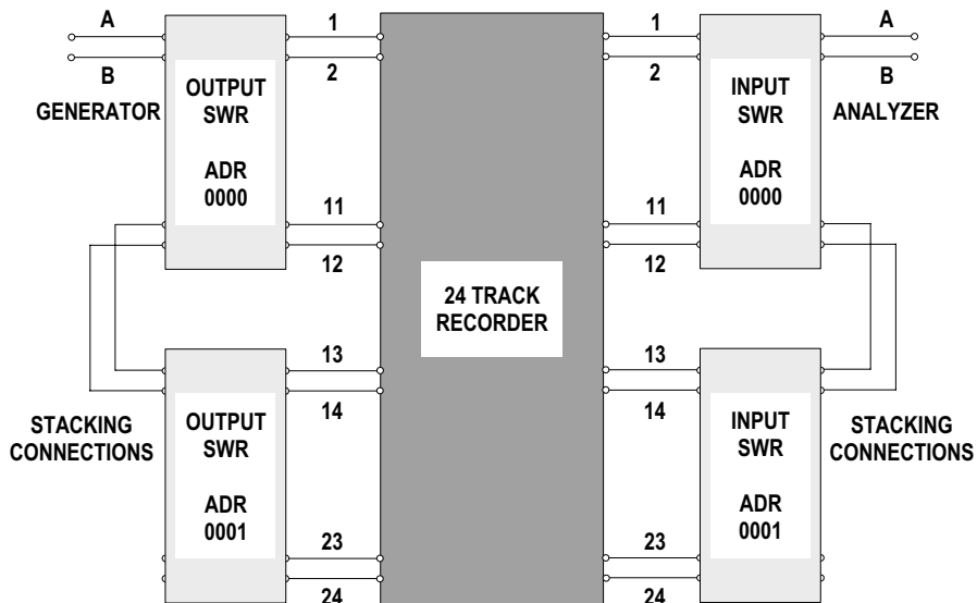
Figure 25-2 Switcher Connection and Address Setting Diagram, Multi-track Recorder
