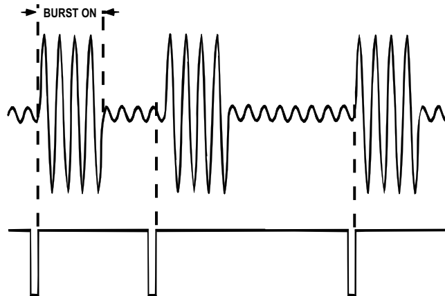
Figure 4-6 Burst Triggered Mode, Definitions
