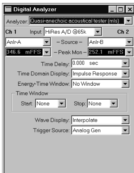
Figure 17-1 MLS Panel, large form
