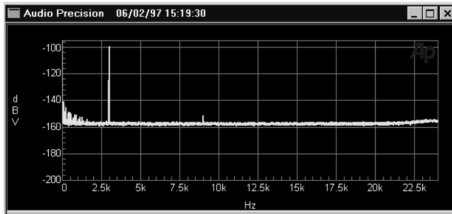
Figure 15-7 Same Low Level Signal, 128x Power (Spectrum only) Averaging. Noise Variance is Reduced, No Change in Average Noise Level
