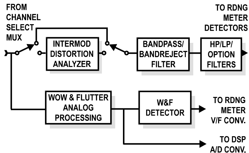
Figure 5-21 System Two Analog Analyzer, Simplified Block Diagram of Function
