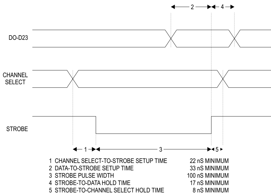
Figure 9-2 Parallel Input Port, Timing Relationships
