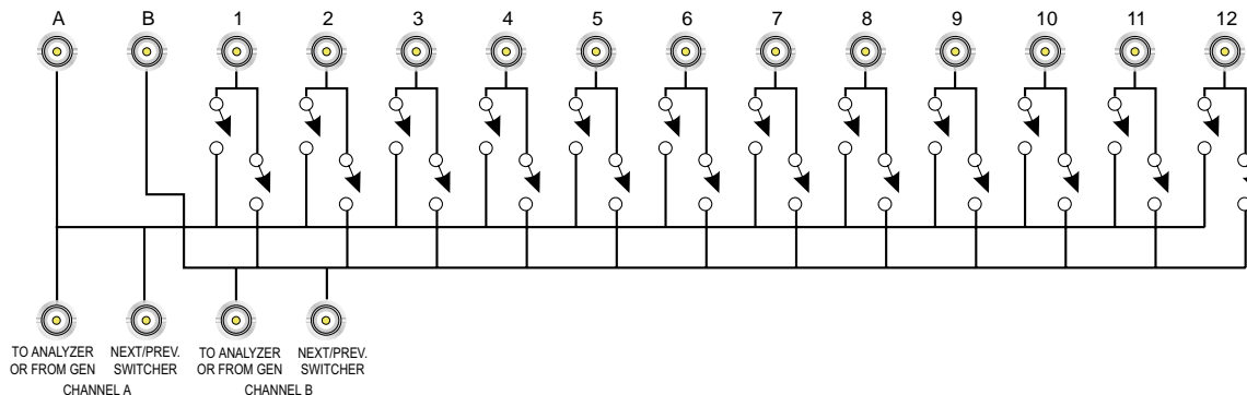
Figure 25-11 SWR-2122U Unbalanced Switcher simplified schematic
