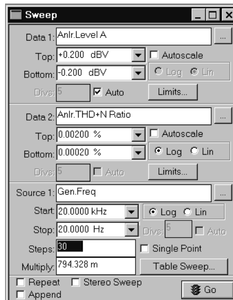
Figure 20-1 Sweep Panel, Small Version
