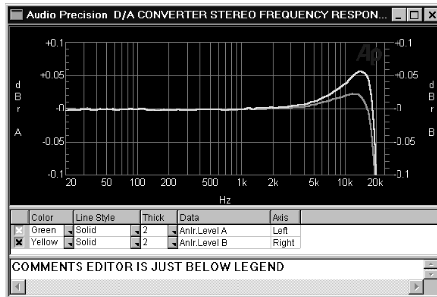
Figure 21-6 Comments Editor
