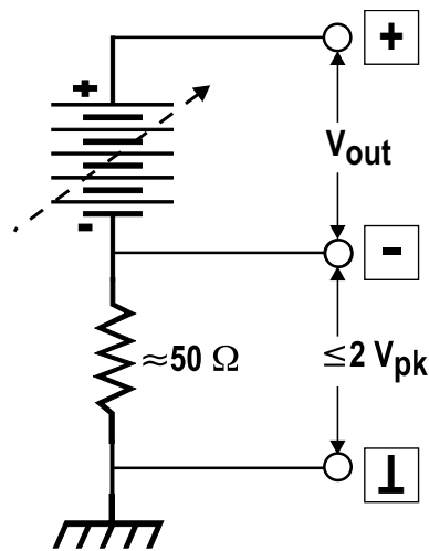
Figure 26-7 Equivalent Circuit, DC Outputs 1 or 2
