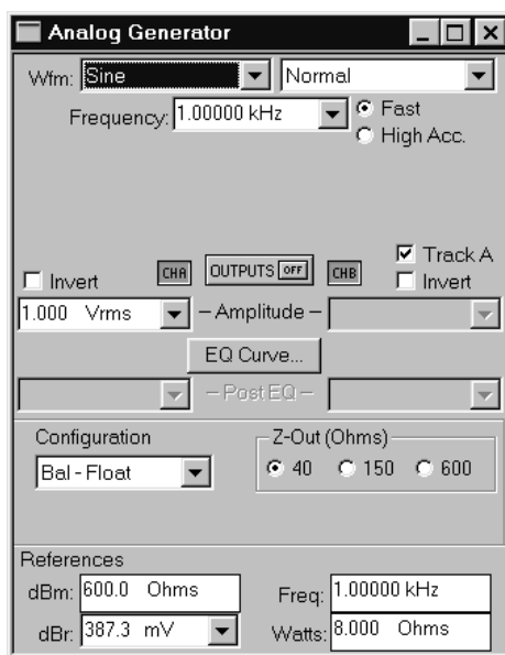
Figure 4-2 Analog Generator Panel, Large Version
