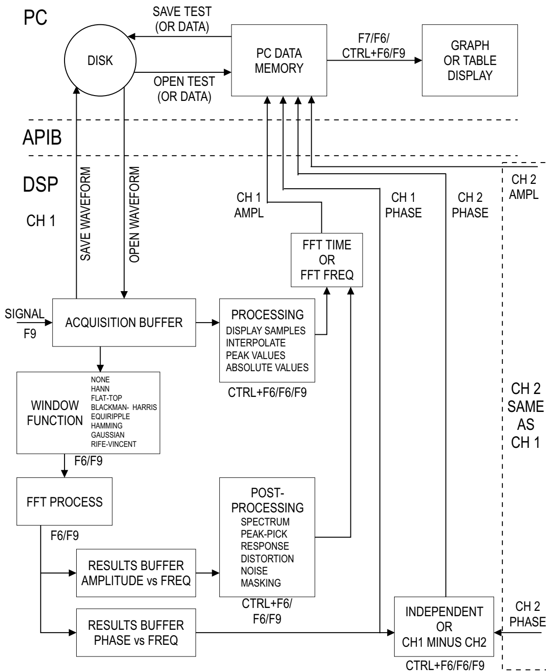
Figure 14-1 Function Block and Process Diagram, System Two FFT Programs
