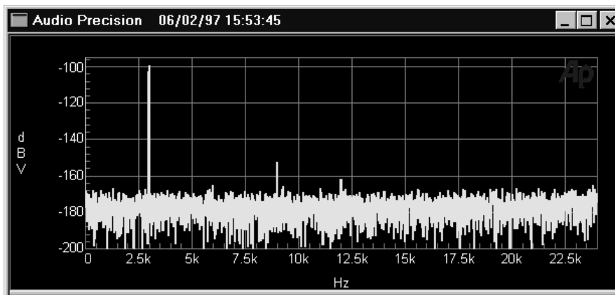
Figure 15-8 Same Low Level Signal, 128x Synchronous (Time Domain) Averaging. Average Noise Level is Reduced, No Change in Noise Variance
