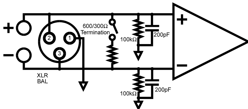
Figure 5-19 System Two Analyzer Equivalent Input Circuit, Balanced XLR
